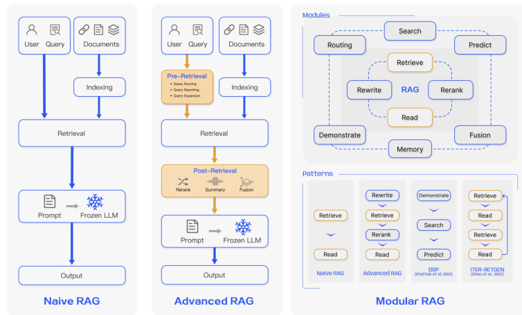
Figure 3.23: Comparison between the three paradigms of RAG [2].
