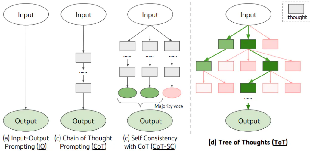
Figure 3.17: Tree-of-Thought (ToT) Framework [64]
