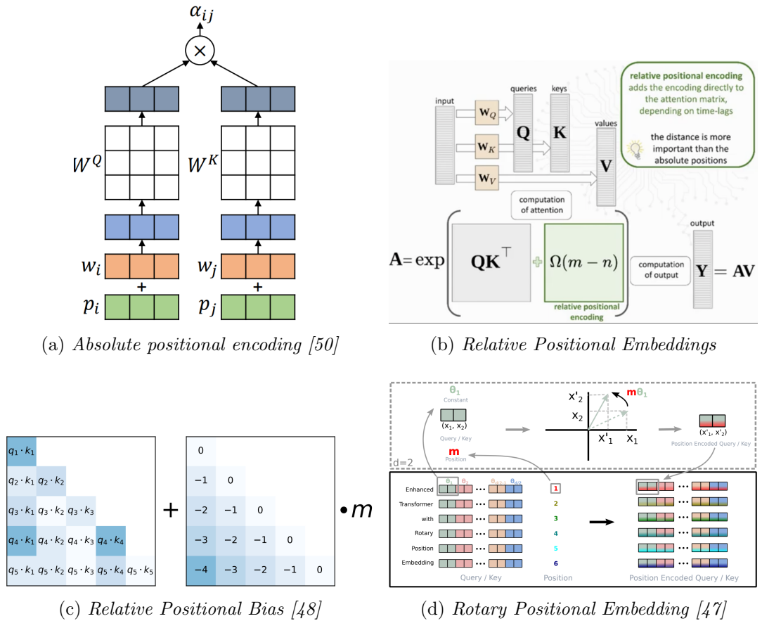
Figure 3.13: Various positional encodings employed in LLMs
