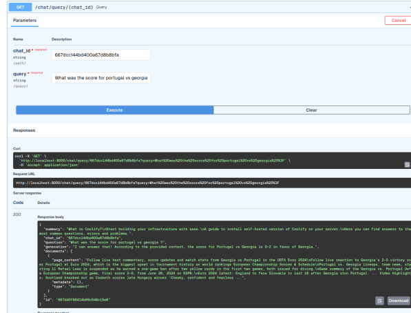
Figure 4.9: 'What was the score of Portugal vs Georgia?' question results.
