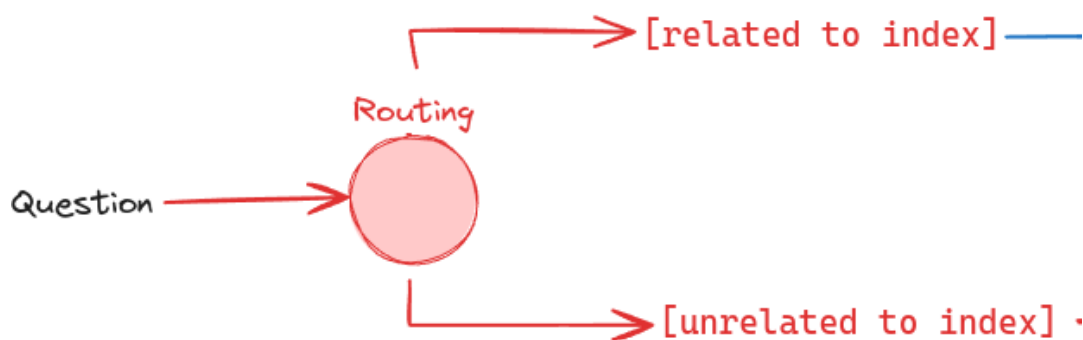
Figure 4.3: Question Routing
