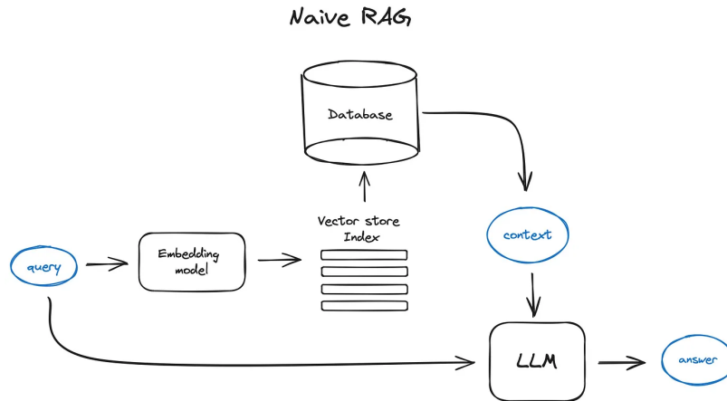
Figure 3.24: Naive RAG
