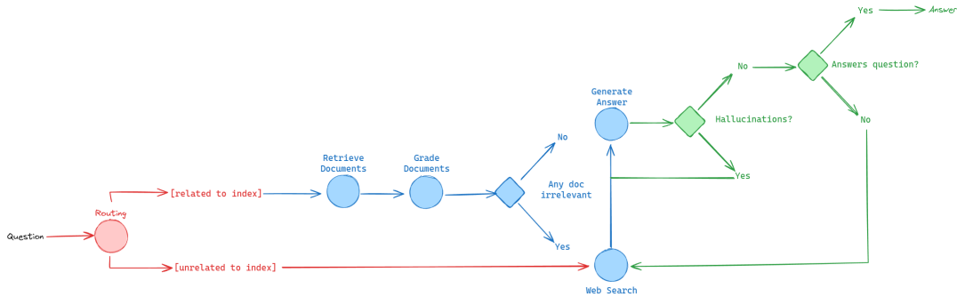
Figure 4.1: Proposed solution architecture.
