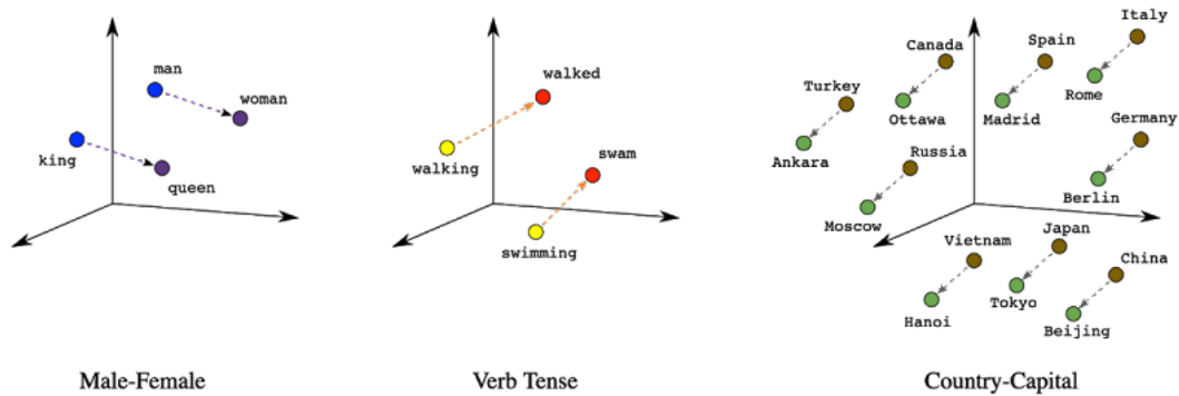
Figure 3.26: Words plotted in 3-dimensional space. Embeddings can have hundreds or thousands of dimensions-too many for humans to visualize [82].
