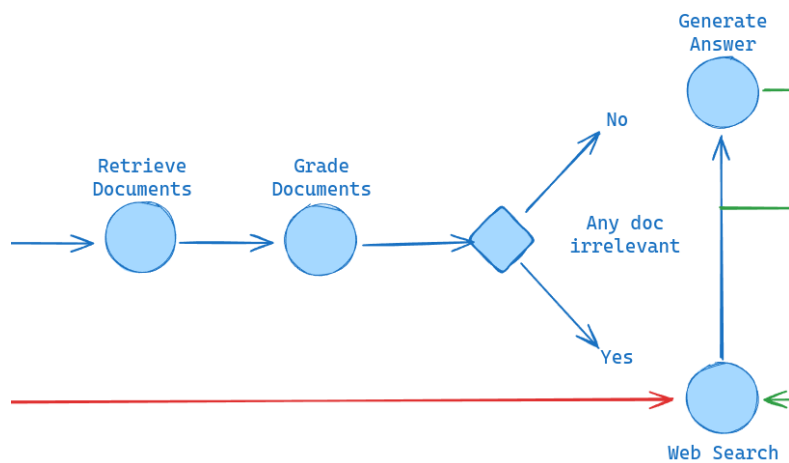
Figure 4.4: Document Retrieval and Grading
