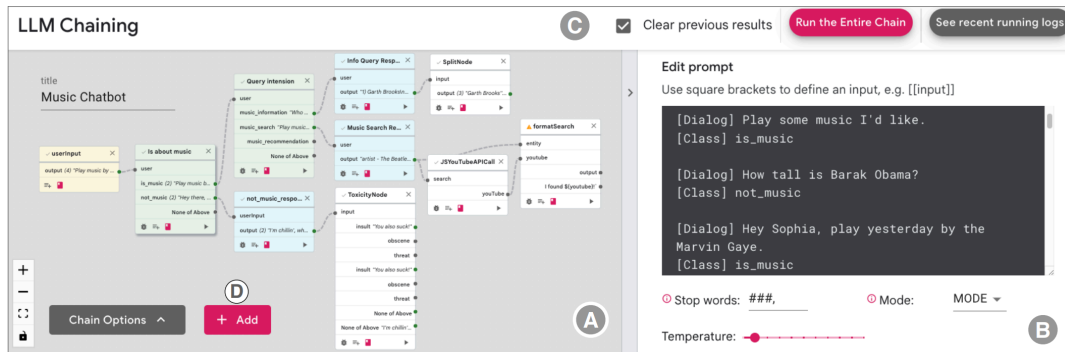
Figure 3.19: The PromptChainer interface. (A) The Chain View visualizes the chain structure with node-edge diagrams (enlarged in Figure 2), and allows users to edit the chain by adding, removing, or reconnecting nodes. (B) The Node View supports implementing, improving, and testing each individual node, e.g., editing prompts for LLM nodes. PromptChainer also supports running the chain end-to-end (C) [67].
