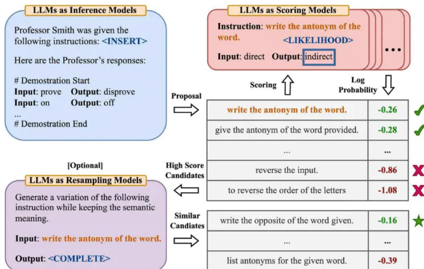
Figure 3.20: Automatic Prompt Engineer framework [68].
