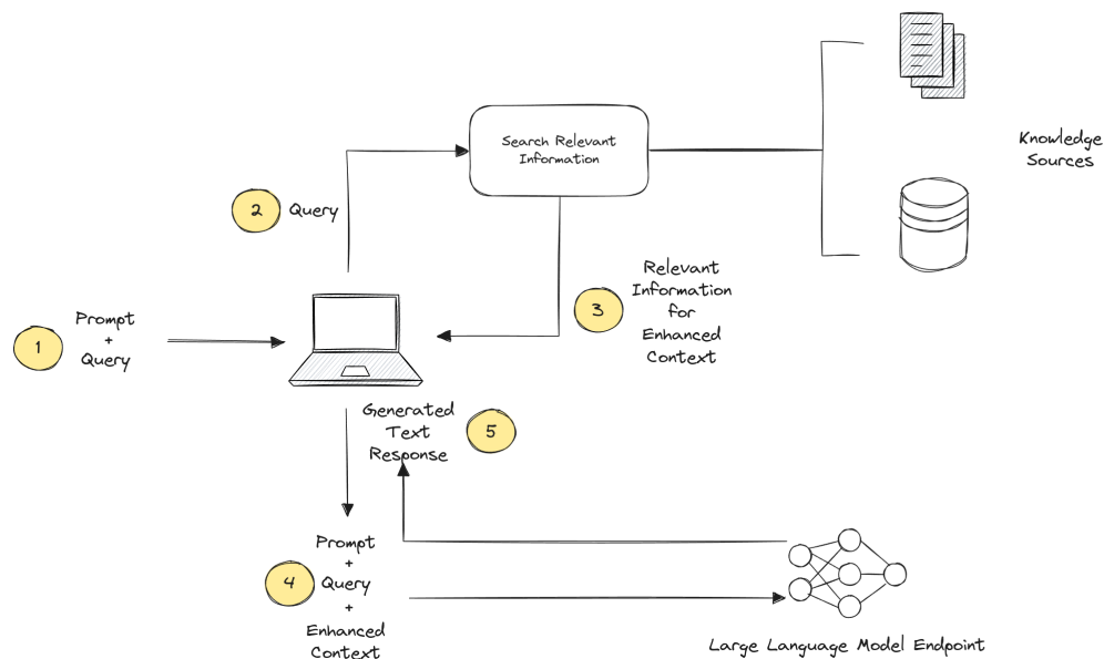
Figure 3.21: An example of synthesizing RAG with LLMs for question answering application.
