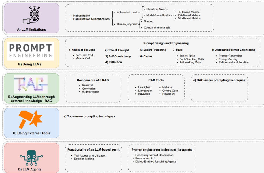
Figure 3.15: How LLMs Are Used and Augmented [45].
