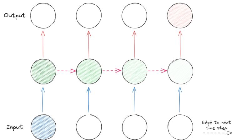
Figure 3.7: Visualization of the vanishing gradient problem, which is indicated by the hidden neuron color fading away [13].
