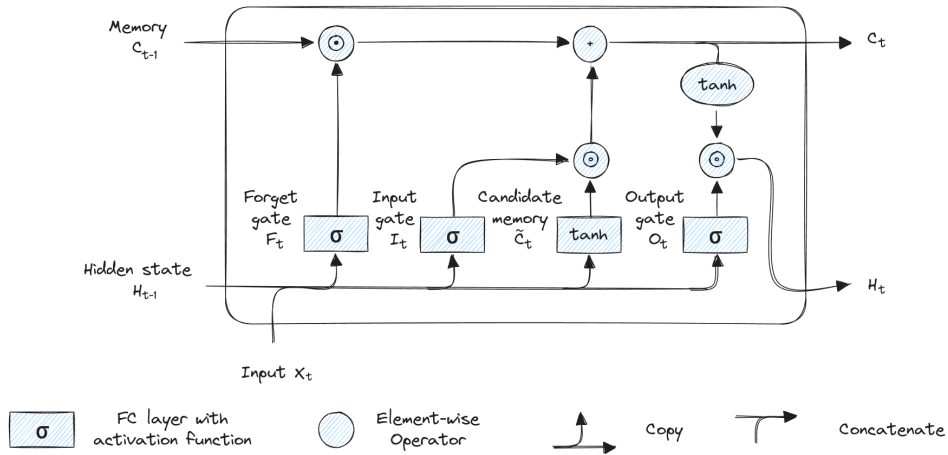
Figure 3.8: Visualization of an LSTM memory cell [16].
