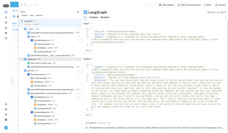
Figure 4.6: Logging and Monitoring with LangSmith.
