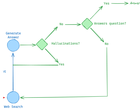
Figure 4.5: Answer validation and correction.
