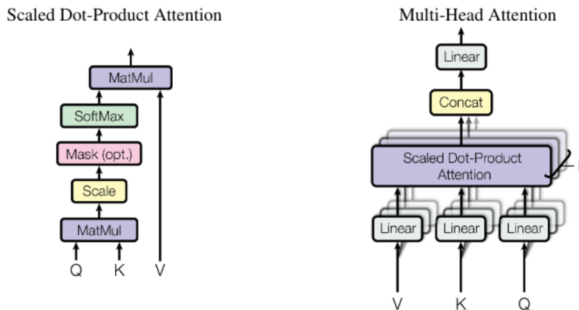
Figure 3.10: Multi-Head attention network [19].
