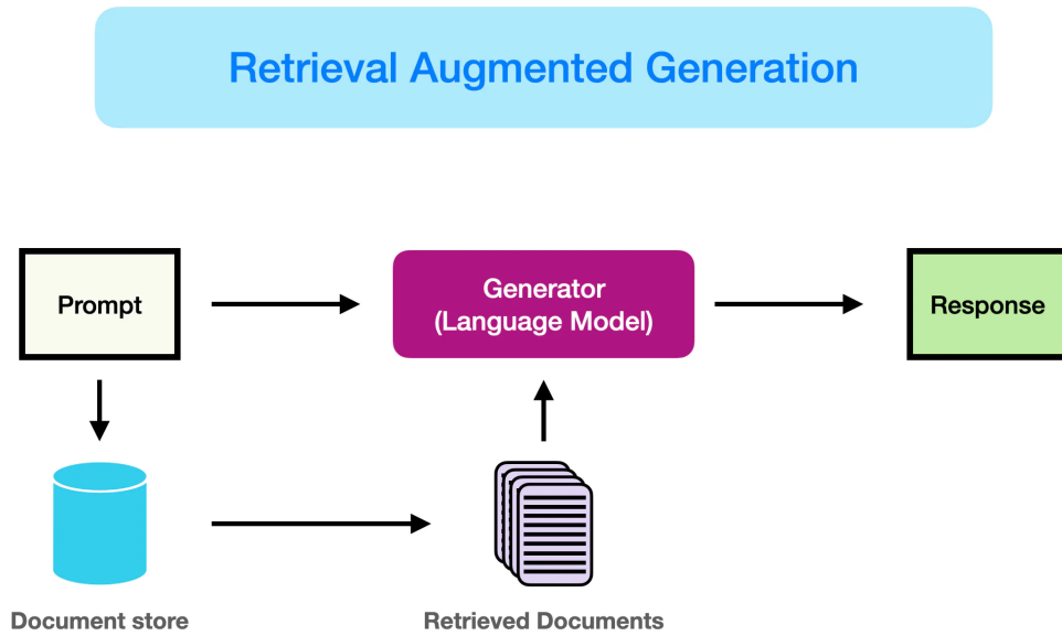
Figure 2.2: Retrieval Augmented Generation.
