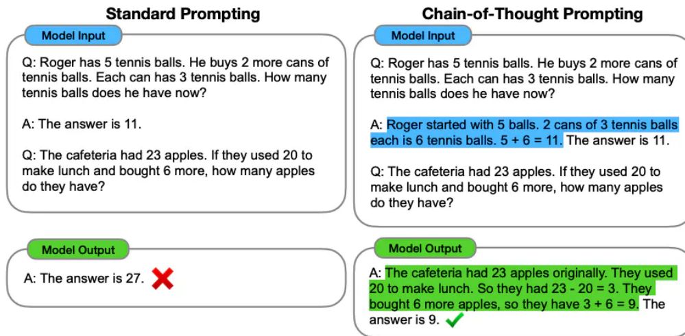
Figure 3.16: Chain-of-Thought (CoT) Prompting [43]
