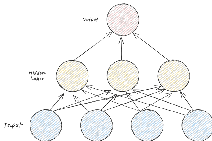
Figure 3.3: Example of a feedforward neural network architecture. The network has an input layer with four neurons, one hidden layer with three neurons and an output layer with a single neuron [13].
