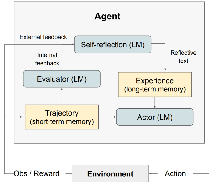
Figure 3.18: Diagram of Reflection [66].
