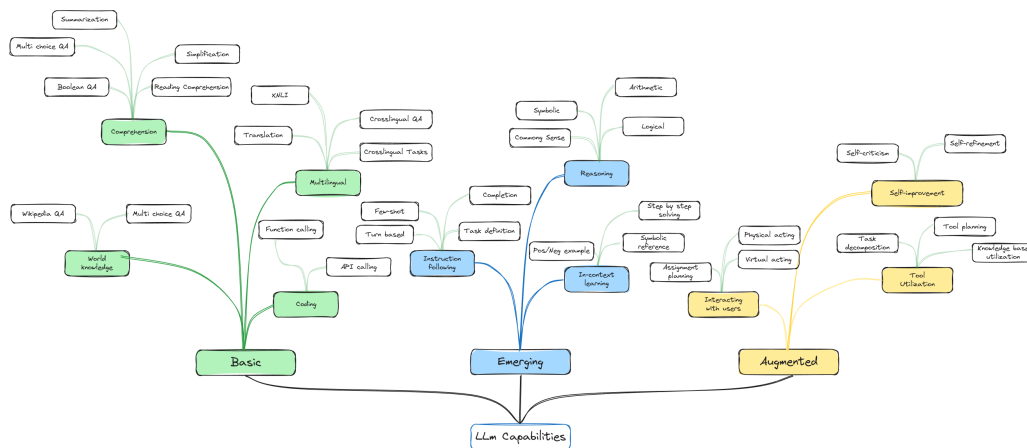
Figure 3.11: LLM capabilities [45]
