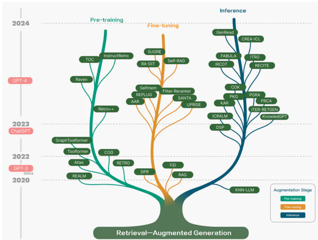
Figure 3.22: Technology tree of RAG research [2]
