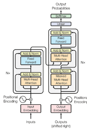
Figure 3.9: Transformer architecture model [19].
