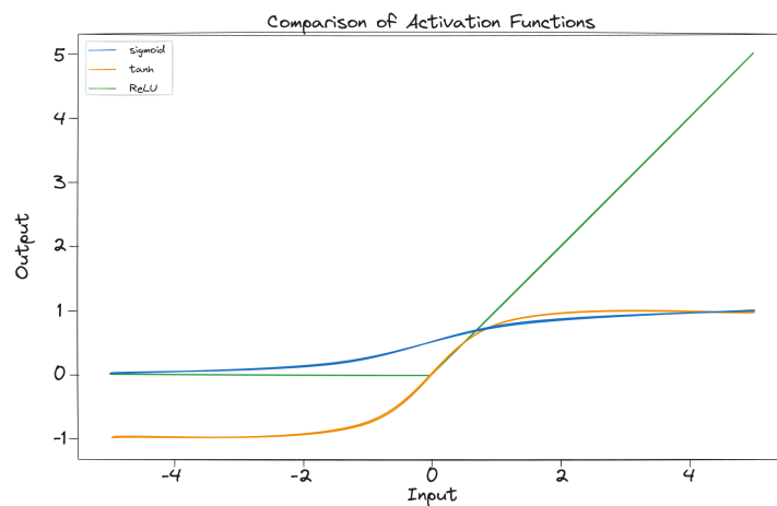
Figure 3.5: Visualization of the sigmoid, tanh and ReLU activation function outputs.
