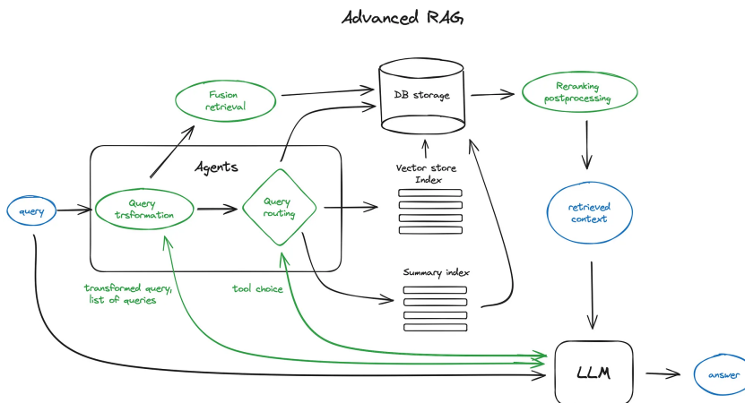
Figure 3.25: Advanced RAG
