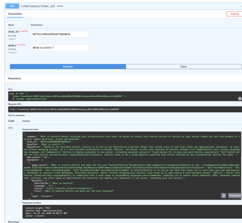
Figure 4.8: 'What is Coolify?' question results.
