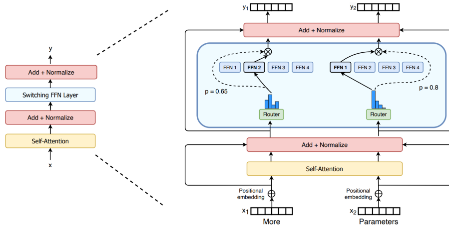
Figure 3.14: Illustration of a Switch Transformer encoder block. They replaced the dense feed forward network (FFN) layer present in the Transformer with a sparse Switch FFN layer (light blue) [52].
